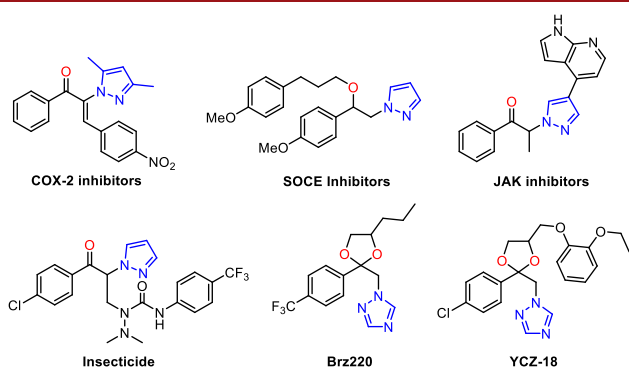
Figure 1. Representative bioactive \alpha -pyrazole ketones.
