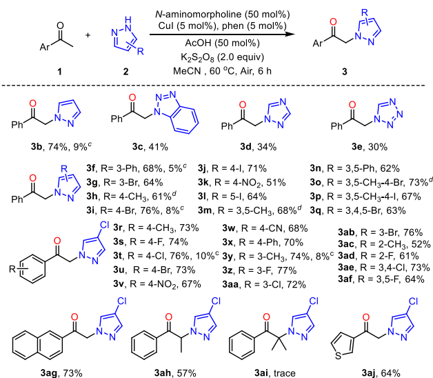
Scheme 2. Selective Monoamination of Ketones a,b
