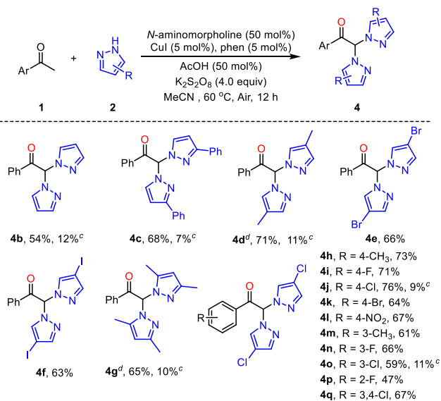
Scheme 3. Selective Diamination of Ketones a,b
